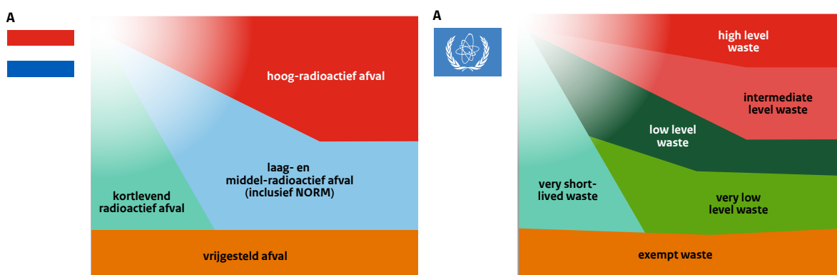
Figure 2: Classification of spent fuel and radioactive waste in Dutch
