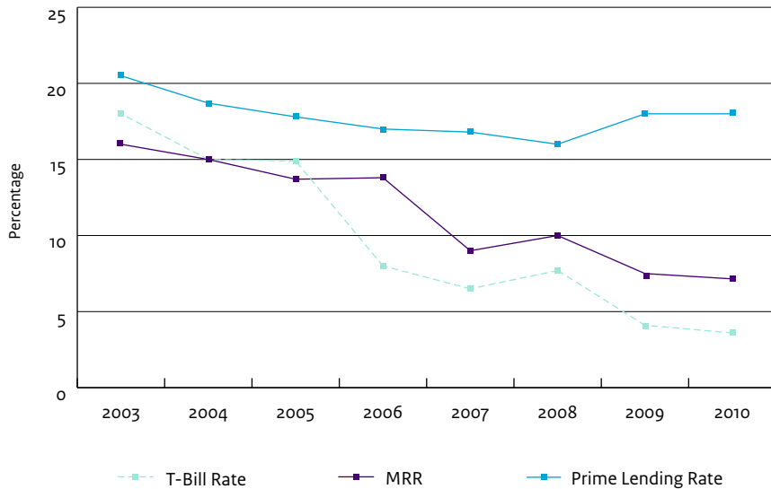
Figure 5.8 Interest rates, in %, annual averages 2003-2010 1,2
