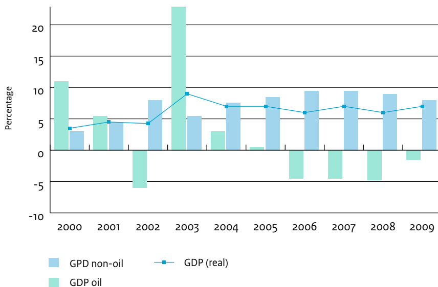
Figure 6.1 GDP growth (oil and non-oil), in %, 2000-2009
