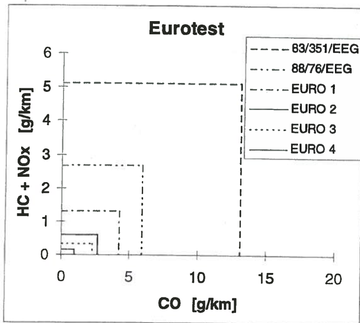
Figure 1: Emission limits on the Eurotest cycle
