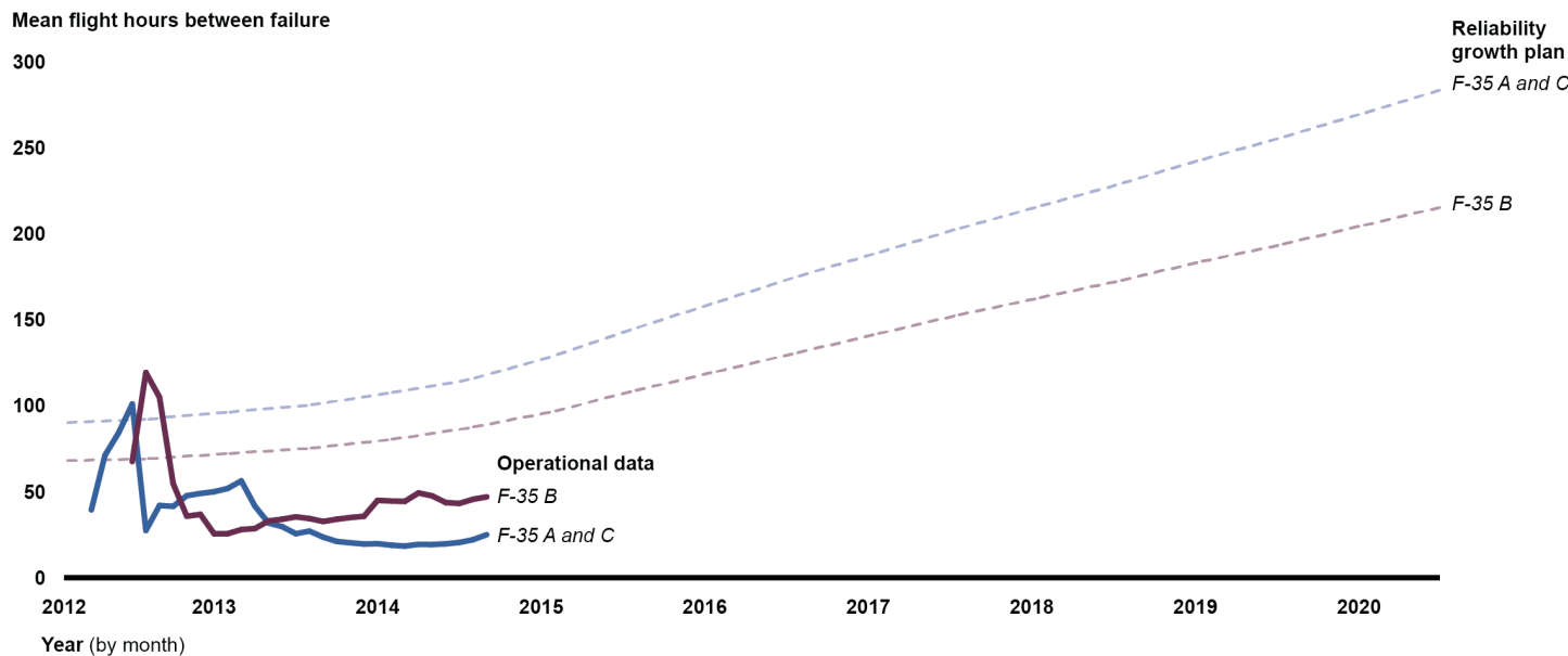
Figure 3: Measured Mean Flight Hours between Failure-(design controlled) for the F-35 Joint Strike Fighter Engine Only
