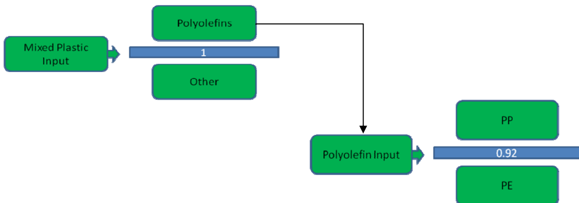
Figure 25 Example of flake sorting of PO by density and secondary polymer separation using a liquid with a density of 0.92g/cm 3
