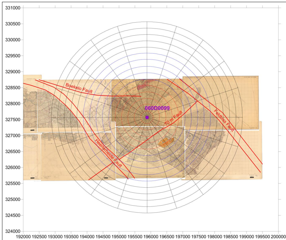
Fig. B 12: The integration net, based on GEERTSMA's influence function, applied for key point 2 (benchmark 060D0099) and coal layer GB36
