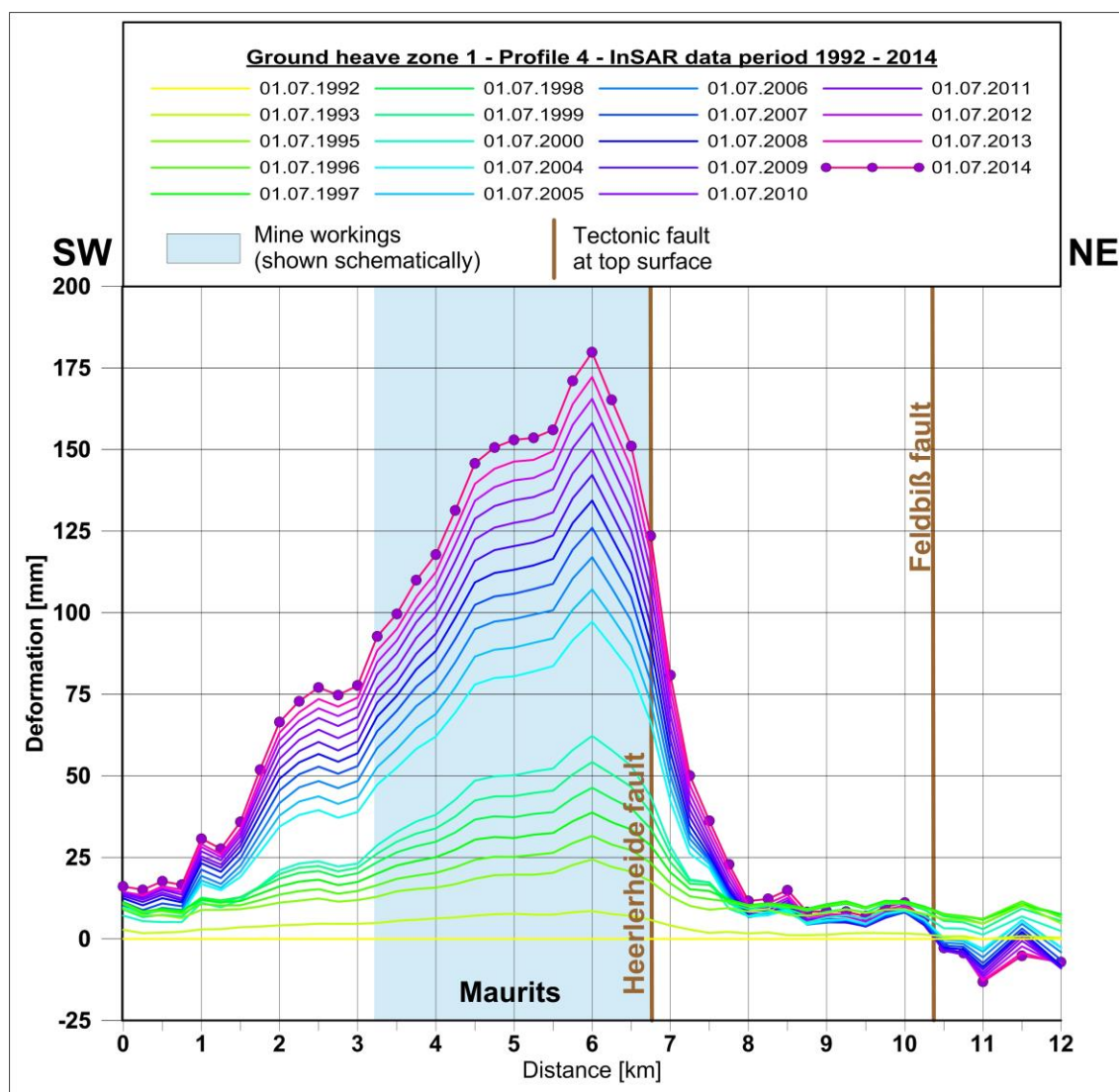
Fig. C 14: Profile 4 SW-NE across the Maurits coal mine (250 m step width)
