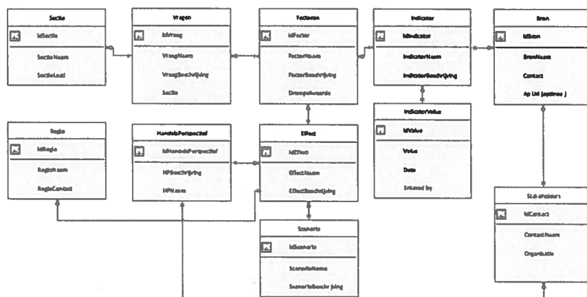
Figure 2 Concept ERD
