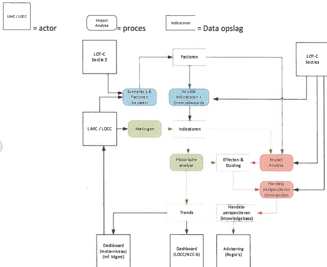
Figure 1 Concept DFD
