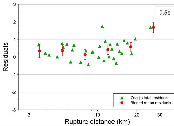
Figure 2.4 Residuals of Sa(T) with respect to the central branch of the GMM V6 at 0.5 seconds.
