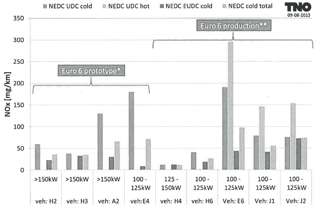
Figure 15: NO x emissions per phase in the NEDC
