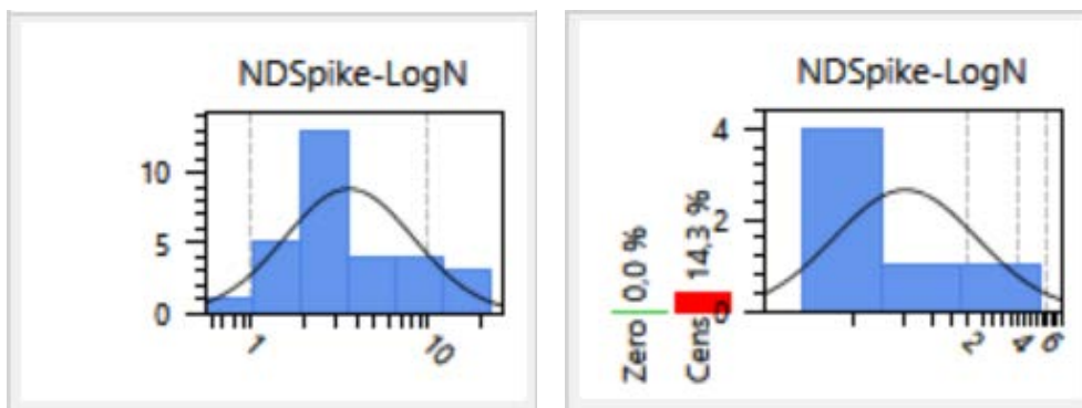
Figure 3. Example of a 'NonDetectSpike LogNormal' distribution fitted to the MOSH concentrations of the food group 'chocolate' (A) (0% non-detect samples) and 'breakfast cereals' (B) (14% non-detect samples)
