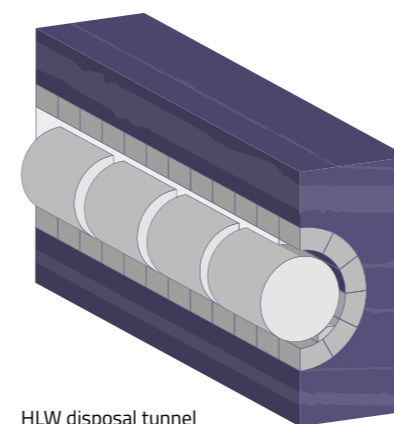
HLW disposal tunnel
