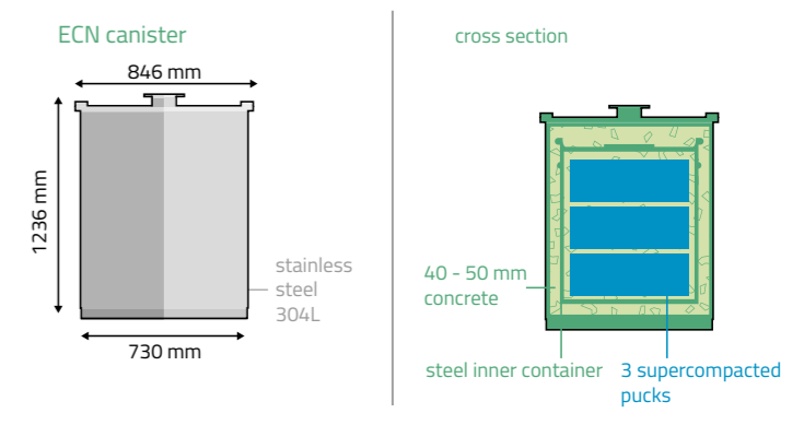
Figure 6-3-9: Schematic of ECN canister with supercompacted pucks of legacy wastes [Verhoef, 2016].
