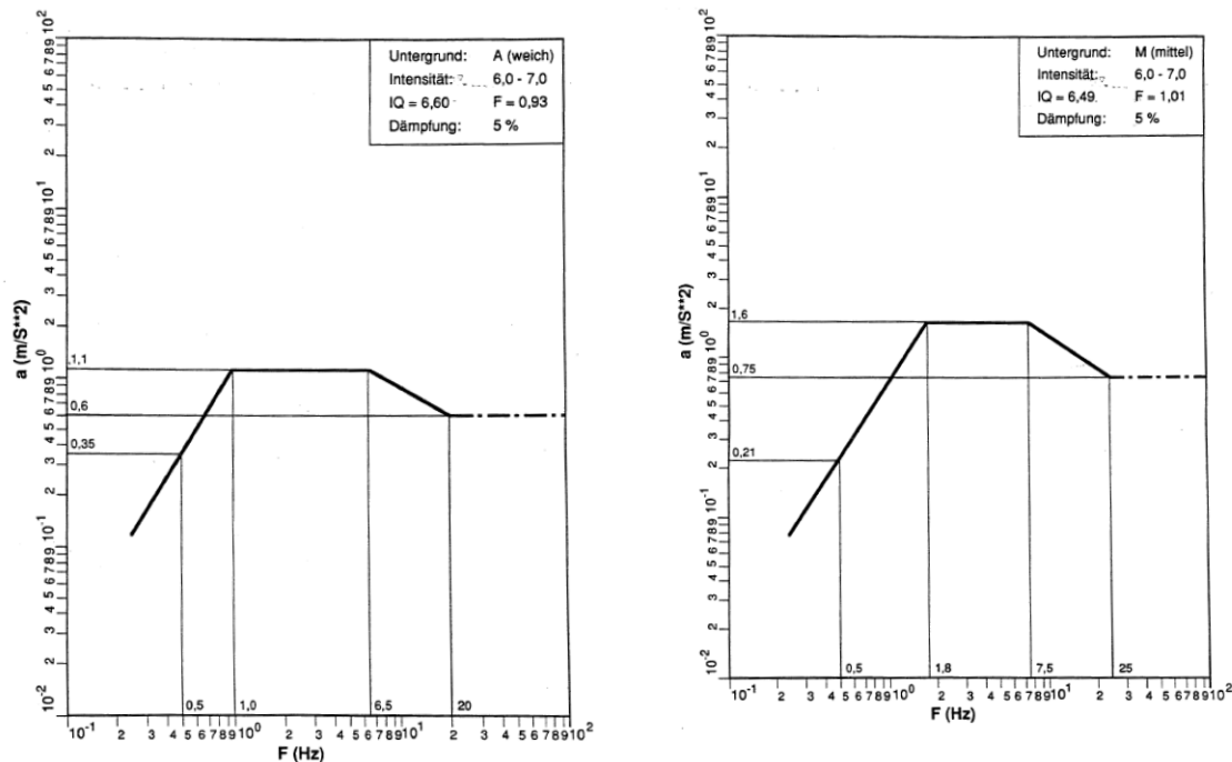
Figure 2-1 Modified ‘Hosser’ spectra used in the second 10-yearly Periodic Safety Review.
