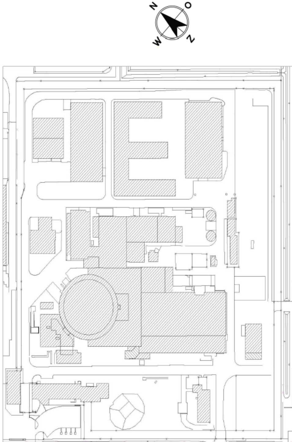
Figure 1-5 Plan of the Borssele NPP and identification of some important buildings 19
