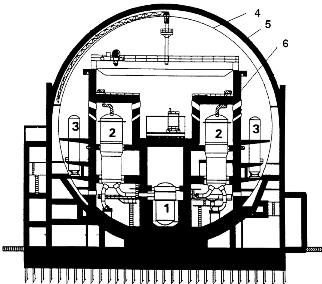
Figure 1-4 Cross section of KCB containment showing a small selection of major components
