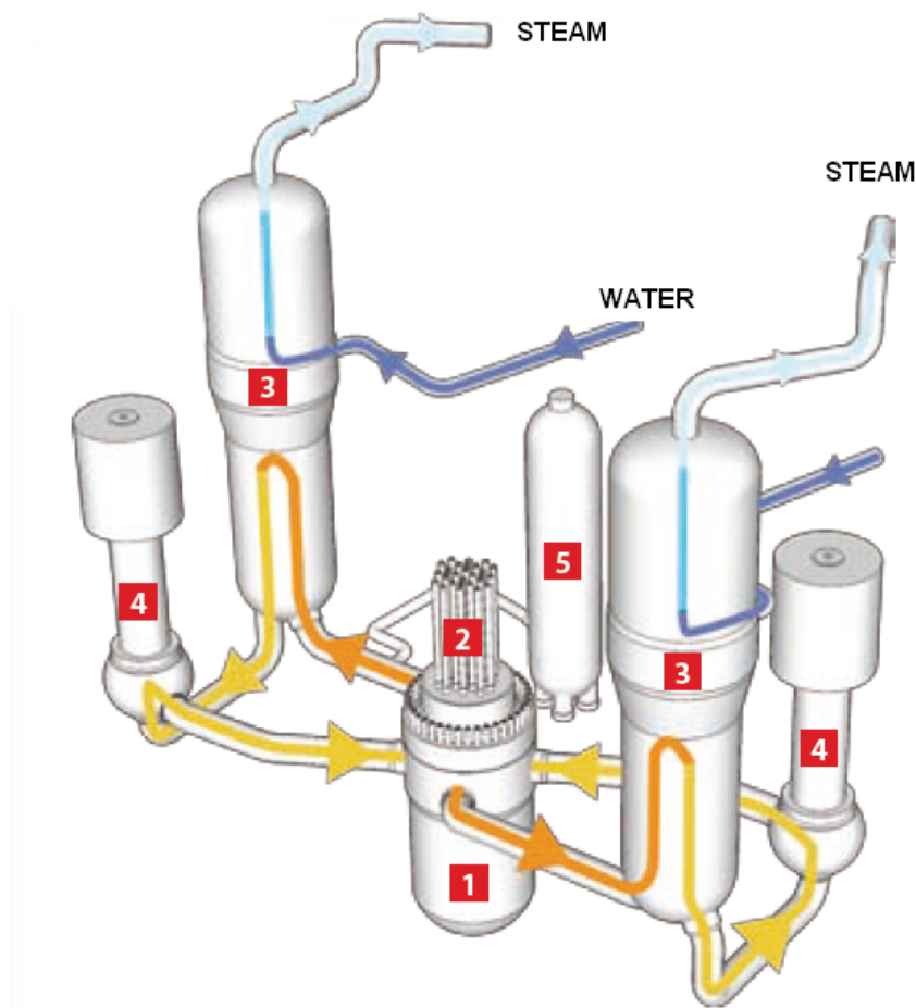
Figure 1-3 Primary system of KCB
