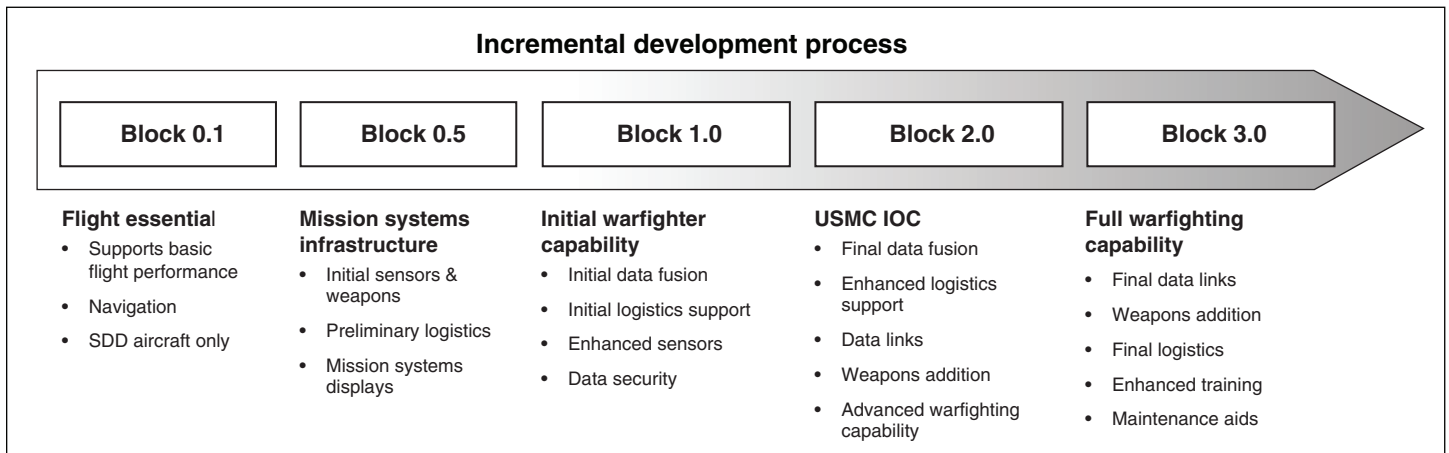
Figure 6: Software Increments
