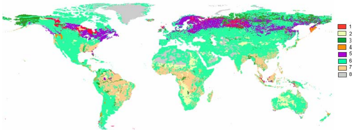
Figure 2: Geographic distribution of soil types. 1=Organic; 2=Sandy Soils; 3=Wetland Soils; 4=Volcanic Soils; 5=Spodic Soils; 6=High Activity Clay Soils; 7=Low Activity Clay Soils; 8=Other Areas
