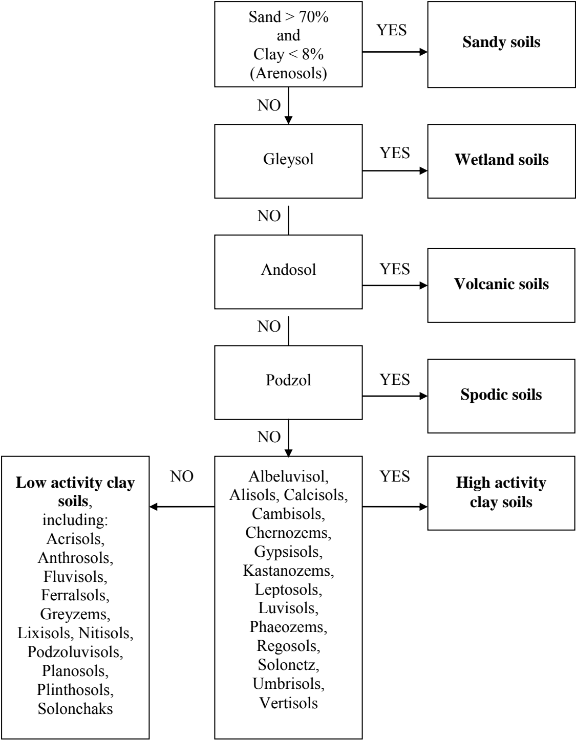
Figure 3: Classification of soil types
