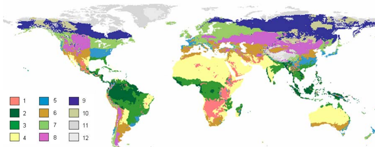
Figure 1: Climate regions. 1=Tropical, montane; 2=Tropical, wet; 3=Tropical, moist; 4=Tropical, dry; 5=Warm temperate, moist; 6=Warm temperate, dry; 7=Cool temperate, moist; 8=Cool temperate, dry; 9=Boreal, moist; 10=Boreal, dry; 11=Polar, moist; 12=Polar, dry;
