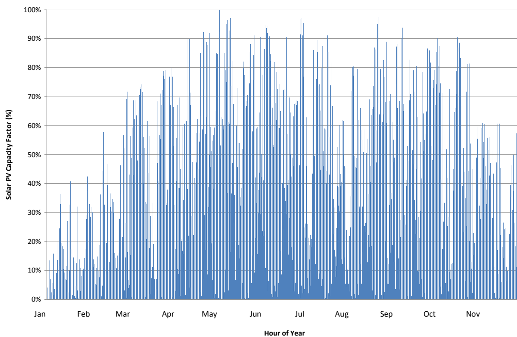
Figure B.3 Solar PV Shape 2011 (Chronological) with capacity factor of 15 percent
