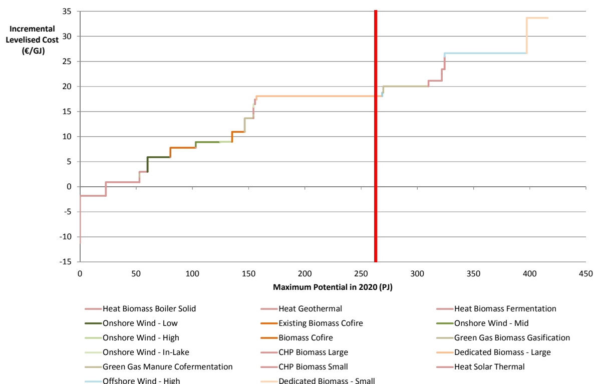
Figure 4.12 2020 Incremental RES Supply Curve (2012 Costs)
