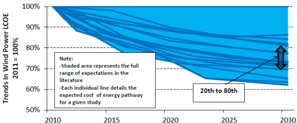
Figure 4.6 Onshore Wind Production Cost Trajectories (IEA, 2012)
