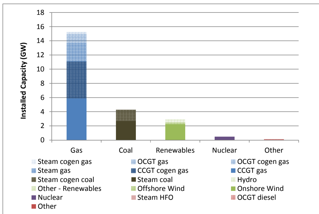
Figure 4.3 Installed Capacity (End of 2011)
