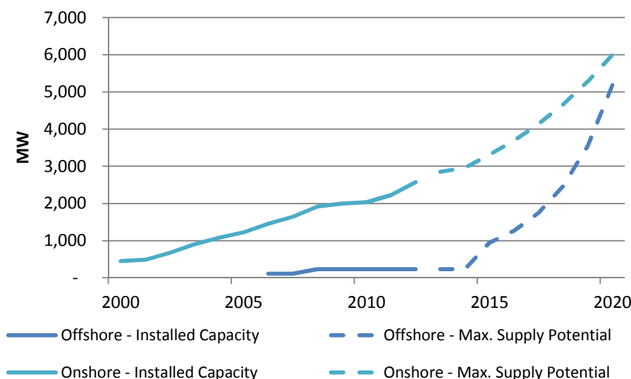
Figure 4.10 Historical Installed Wind Capacity and Future Capacity Constraints
