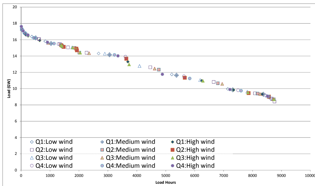
Figure B.5 Selected Bands in Load Duration Curve
