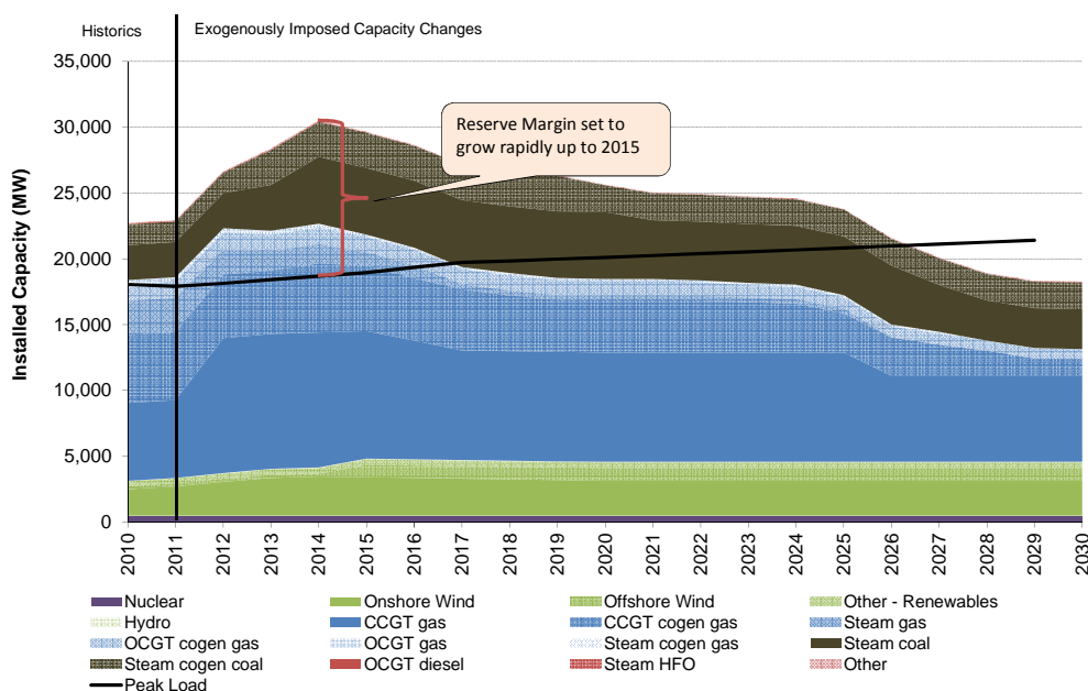
Figure C.2 Exogenously Imposed Capacity Changes
