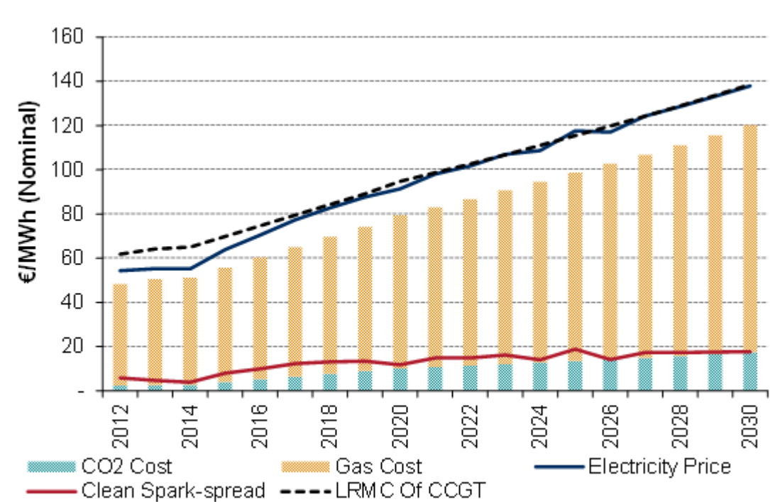
Figure 3.4 Electricity Market: Selected Production Costs, Prices, and Spark Spread
