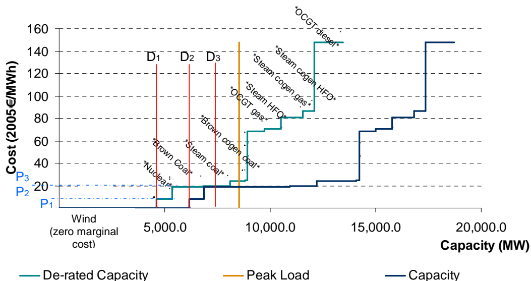
Figure 3.3 Example Supply-Demand Optimization
