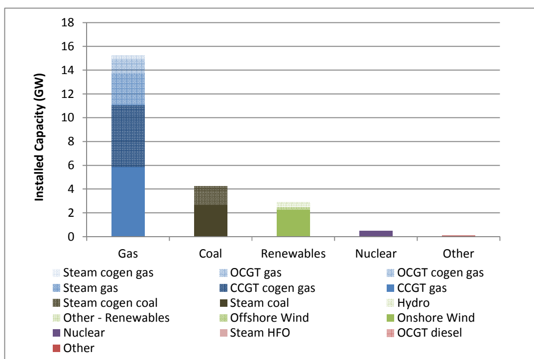
Figure C.1 Installed Capacity (End of 2011)
