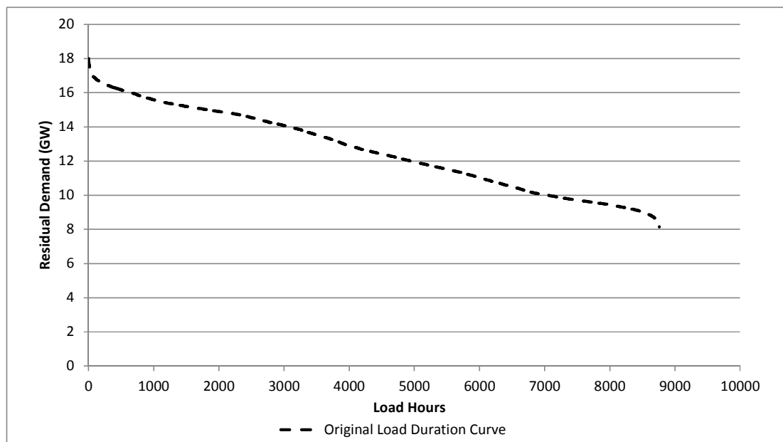
Figure B.4 Original Load Duration Curve
