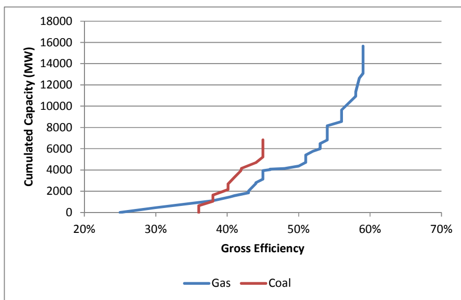
Figure C.3 Distribution of Gross Efficiencies of Gas and Coal Plants
