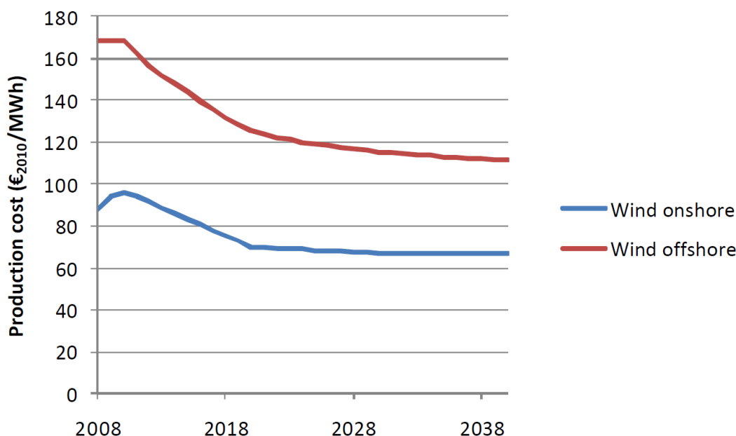
Figure 4.5 Onshore and Offshore Wind Production Cost Trajectories (ECN, 2011)
