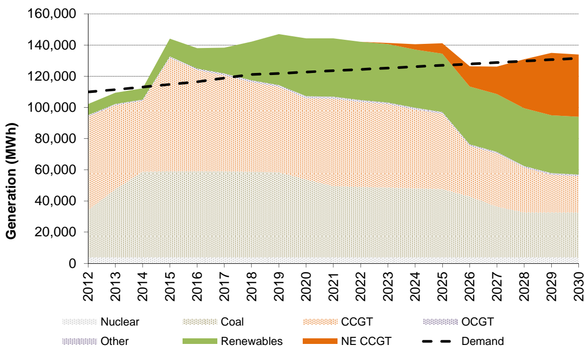
Figure 3.6 Electricity Generation and Demand
