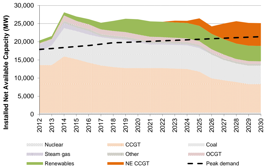
Figure 3.6 Electricity Generation and Demand
