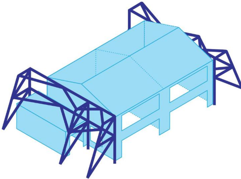
Figure 44 Temporary steel “bookend” frames
