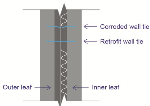
Figure 34 Replacement of corroded cavity wall ties
