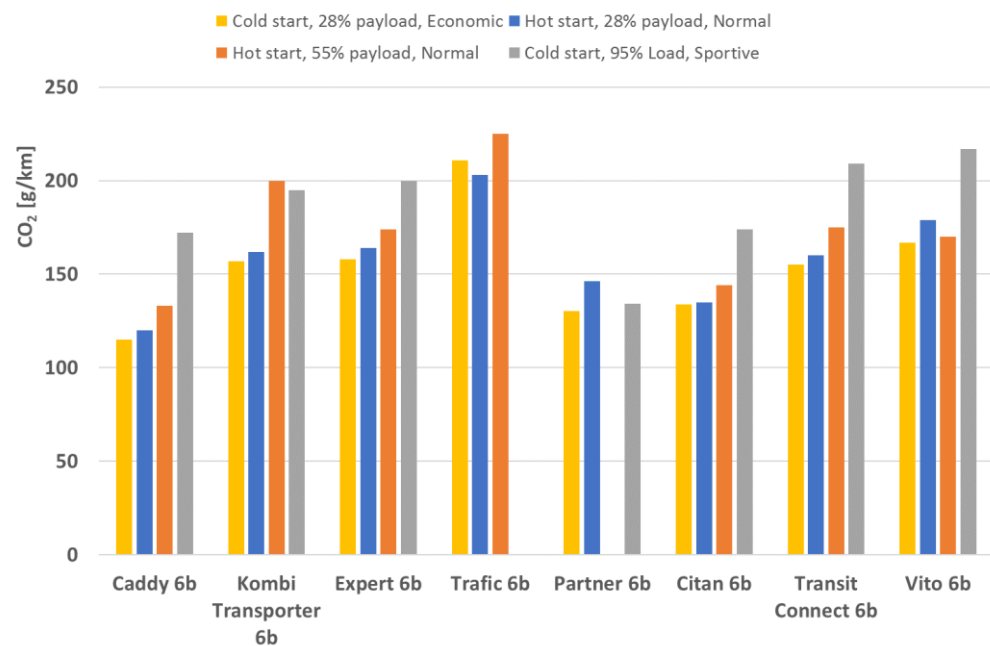
Figure 3-61: CO 2 emissions of RDE trips with different payloads and driving styles of 8 vehicles
