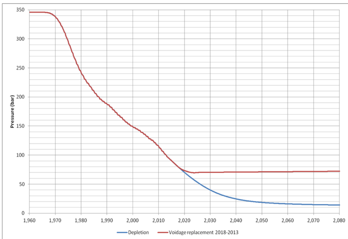
Figure 12.10 Comparison of the pressure development over time for the continued depletion drive development case and the pressure maintenance development based on nitrogen injection. The reservoir pressure for the latter case is stabilised at around 60 - 70 bar.
