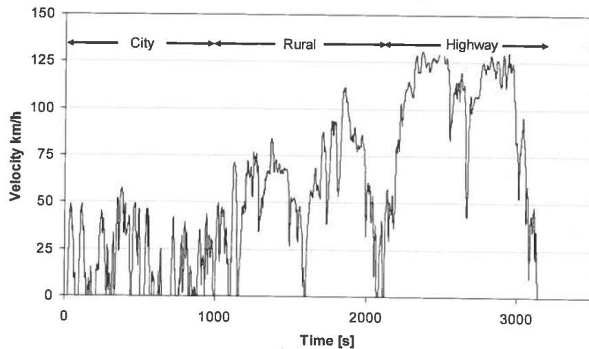
Figure 3: CADC (Common Artemis Driving Cycle).
