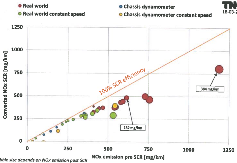
Figure 36: Converted NOx by the SCR of vehicle O1
