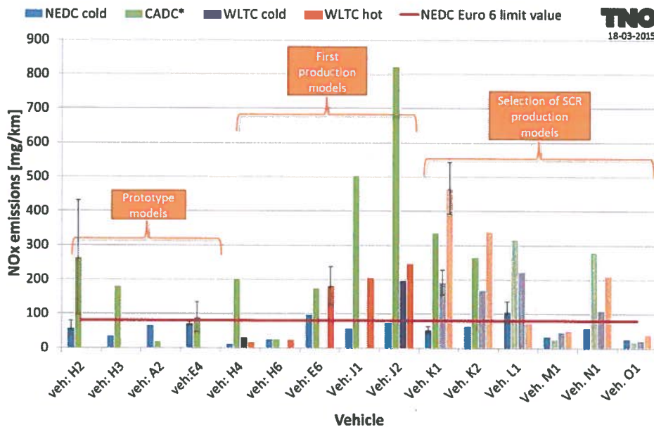
Figure 9: NO x emissions per driving cycle.
