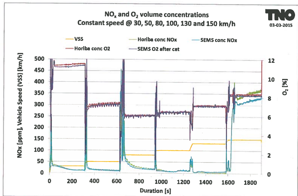
Figure 14: O 2 and NO x volume concentrations with SEMS and chassis dynamometer analysers
