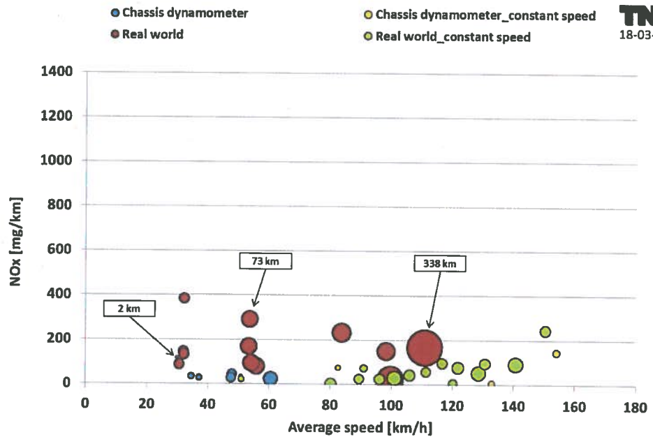
Figure 26: Post-SCR NO x emissions of vehicle O1 of on-road trips and chassis dynamometer tests.
