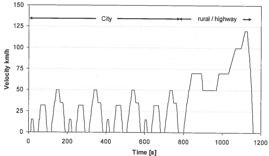
Figure 2: NEDC (New European Driving Cycle).
