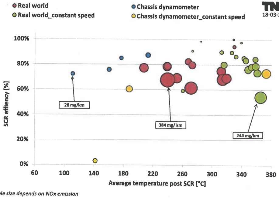
Figure 35: Average SCR operating temperature versus SCR conversion rates of vehicle O1
