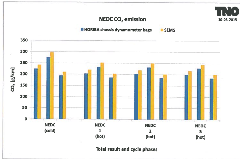
Figure 12: Validation CO 2 test results SEMS-chassis dynamometer.
