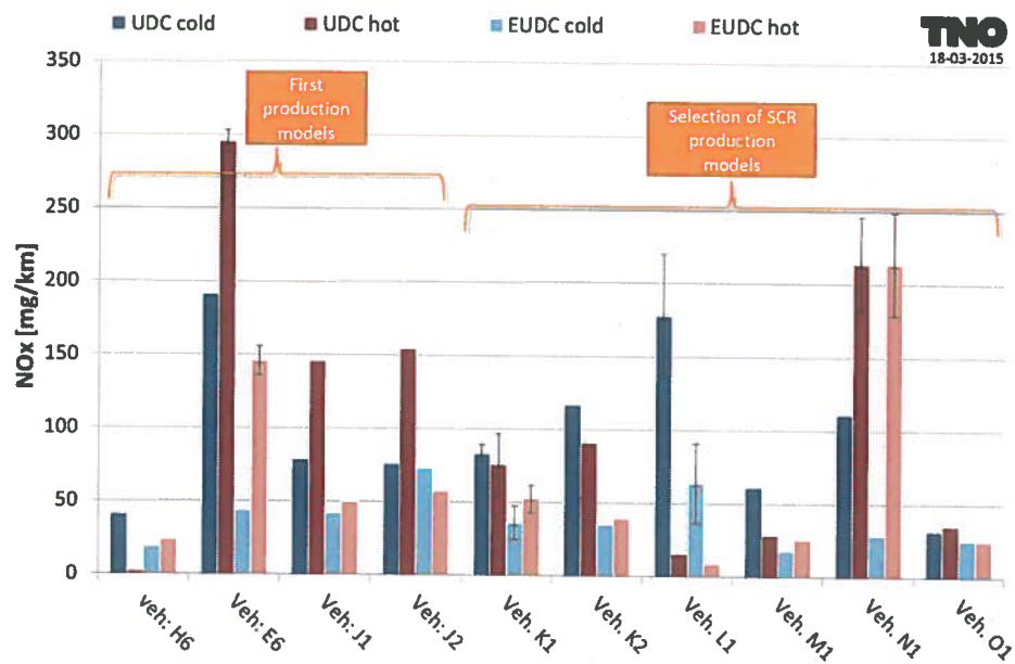
Figure 10: NO x emissions per phase in the NEDC.
