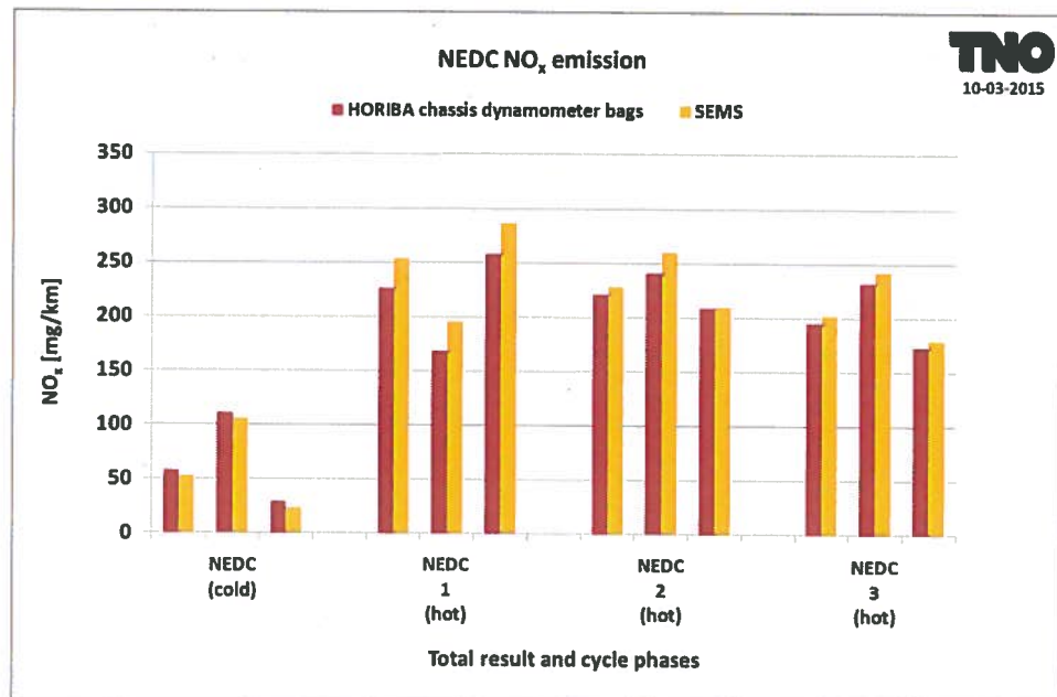
Figure 13: Validation NO x test results SEMS-chassis dynamometer.
