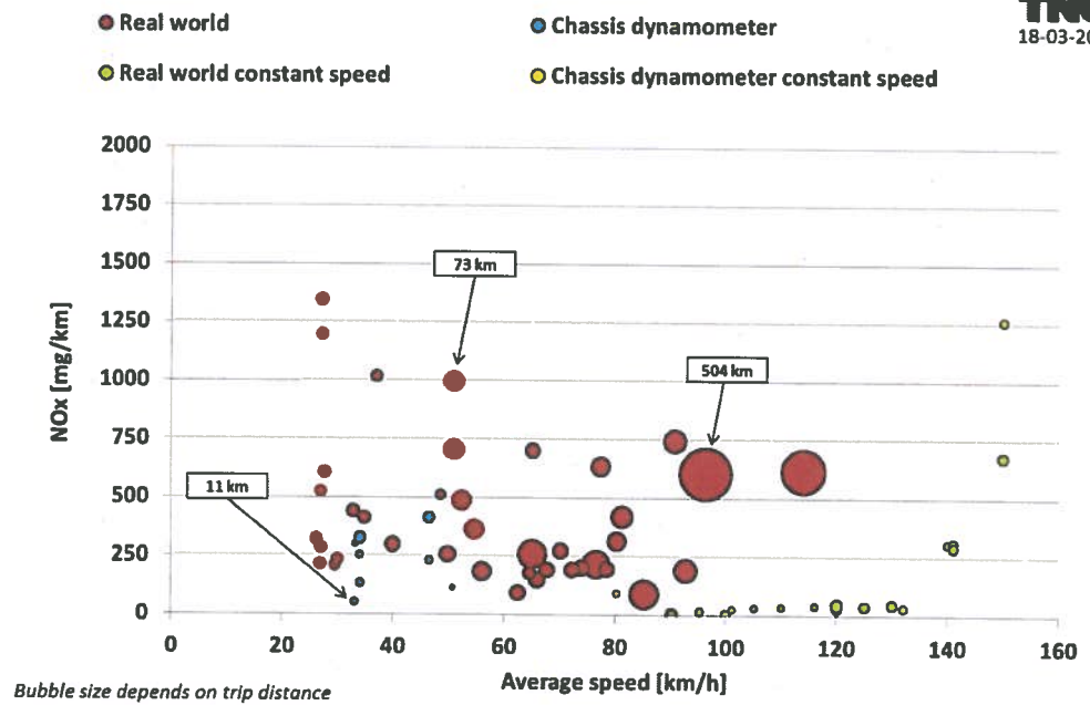
Figure 24: Post-SCR NOx emissions of vehicle N1 of on-road trips and chassis dynamometer tests.
