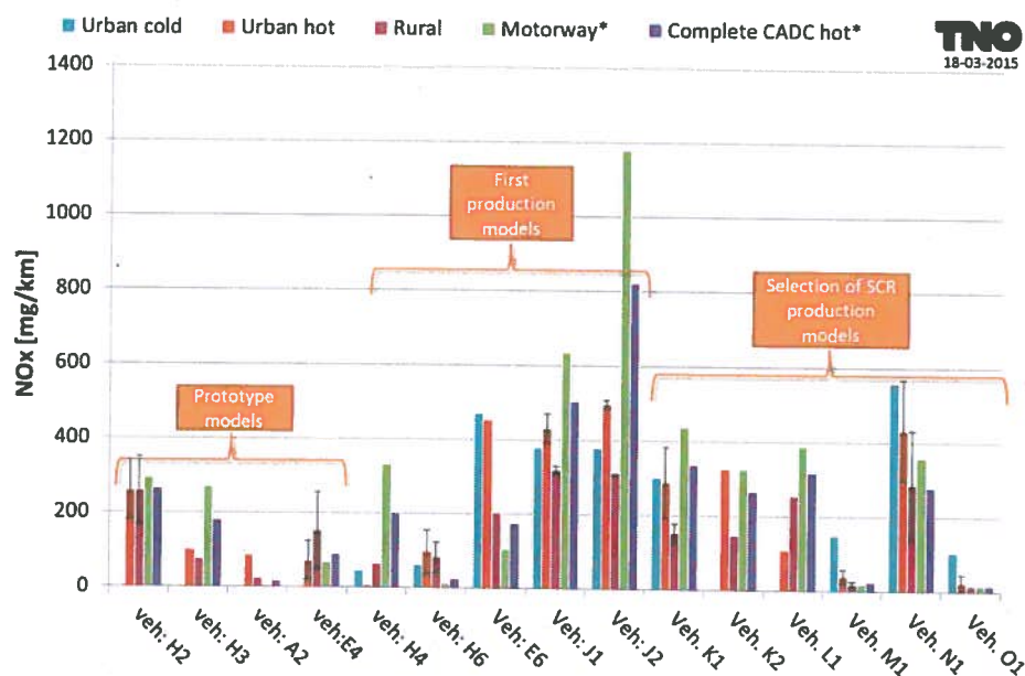
Figure 11: NO x emissions per phase in the CADC.
