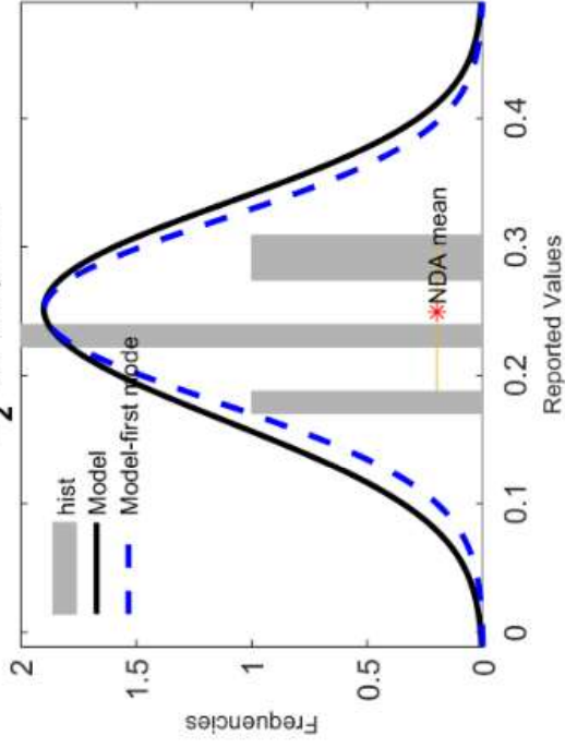
8 2 diPAP, 793
