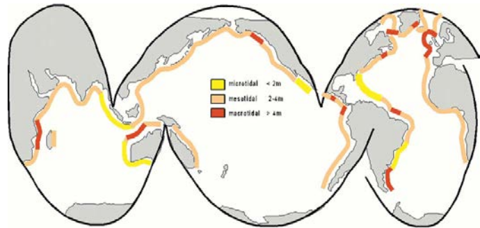
Figure Worldwide distribution of coastal tidal ranges.
