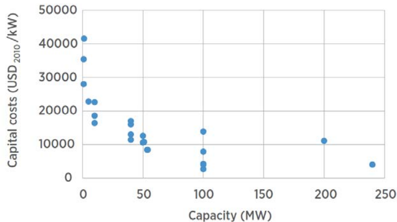
Figure 5: capital cost estimates for OTEC plants
